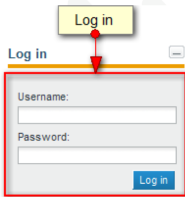
Figure 3: Login page
