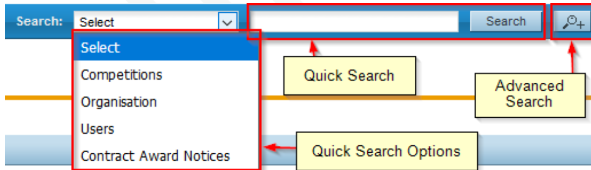
FIGURE 2-1: Search panel
